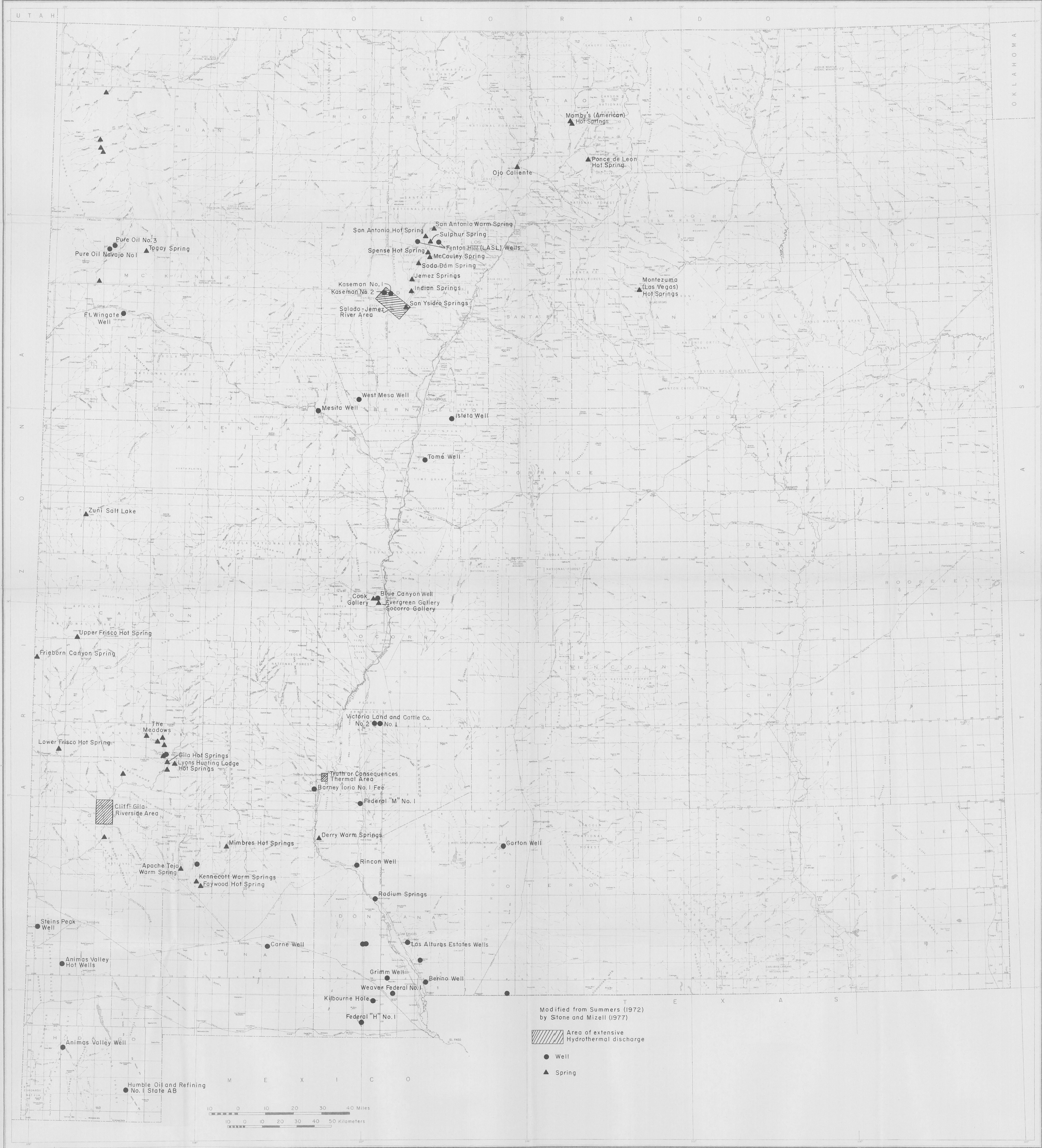
MAP SHOWING LOCATION OF THERMAL SPRINGS, WELLS, AND DISCHARGE SITES IN NEW MEXICO
