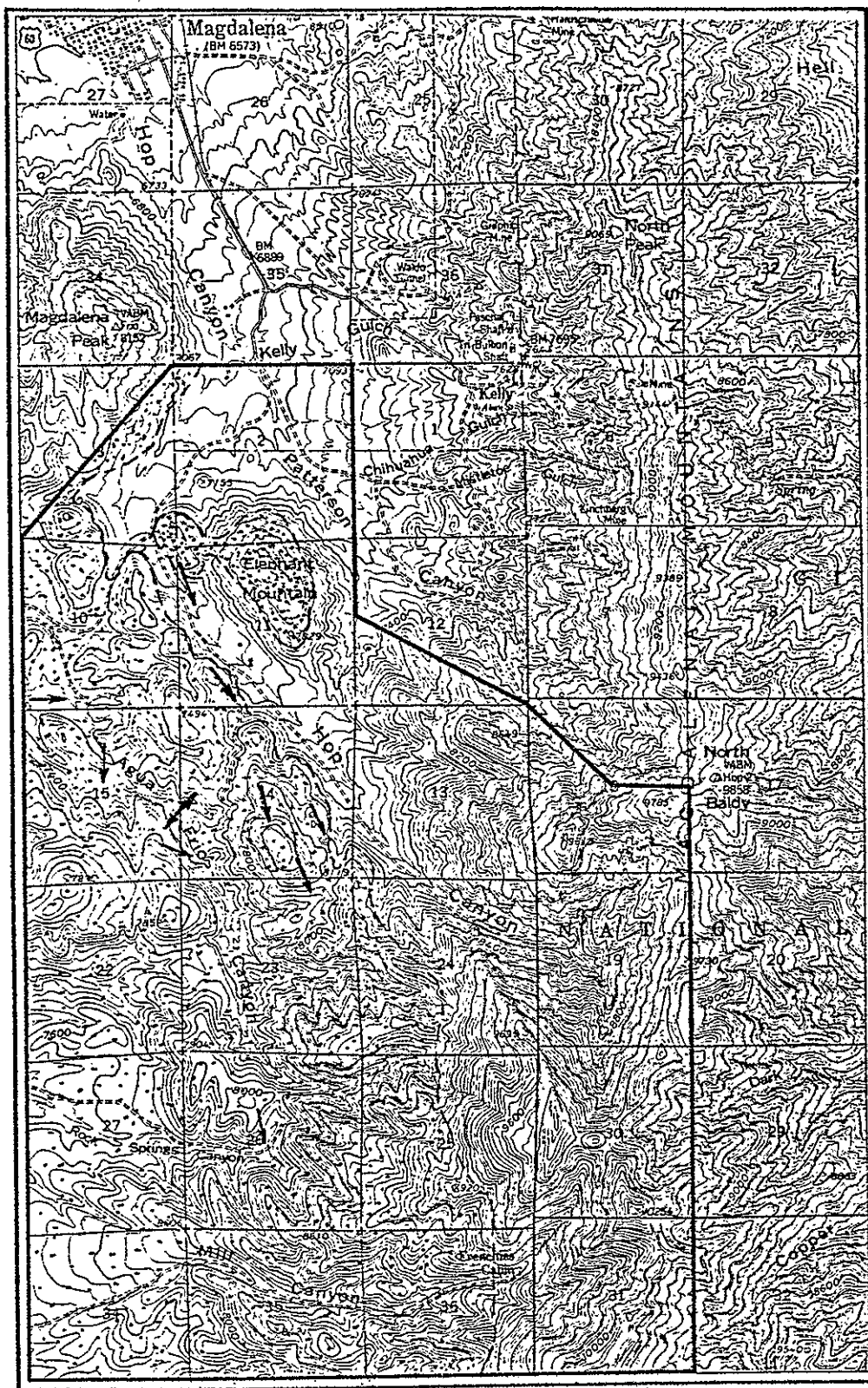
Figure 12. Map showing transport direction of the rhyolite of Magdalena Peak. Transport axis : ↔ . Transport direction : → .
