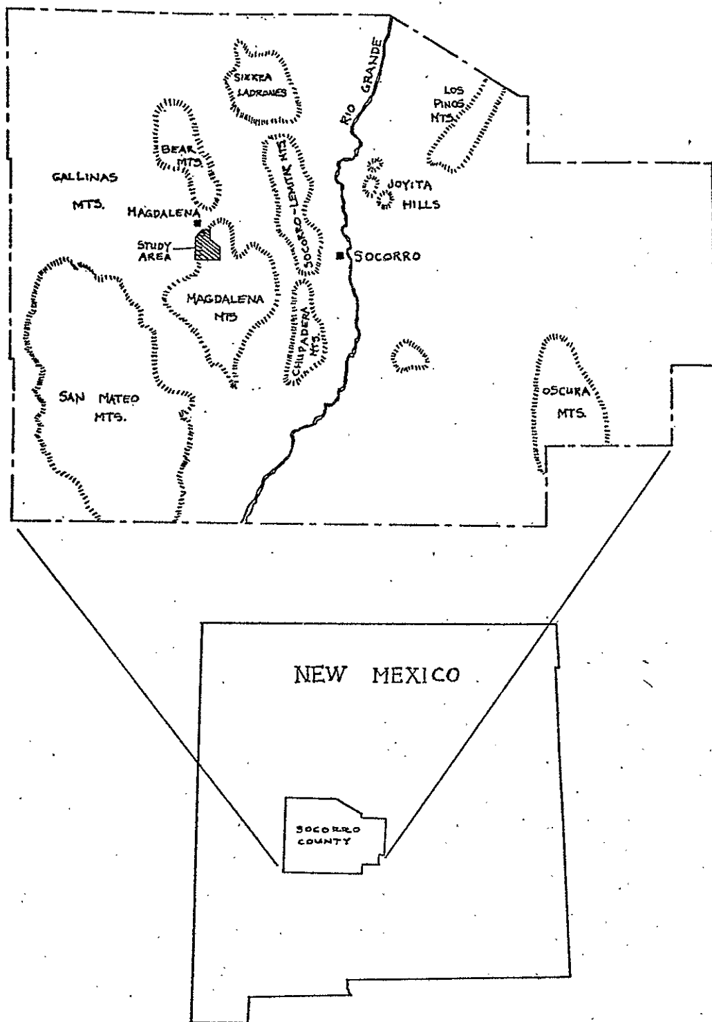
Figure 1. Location map showing relationship of thesis area to major topographic features in Socorro County.
