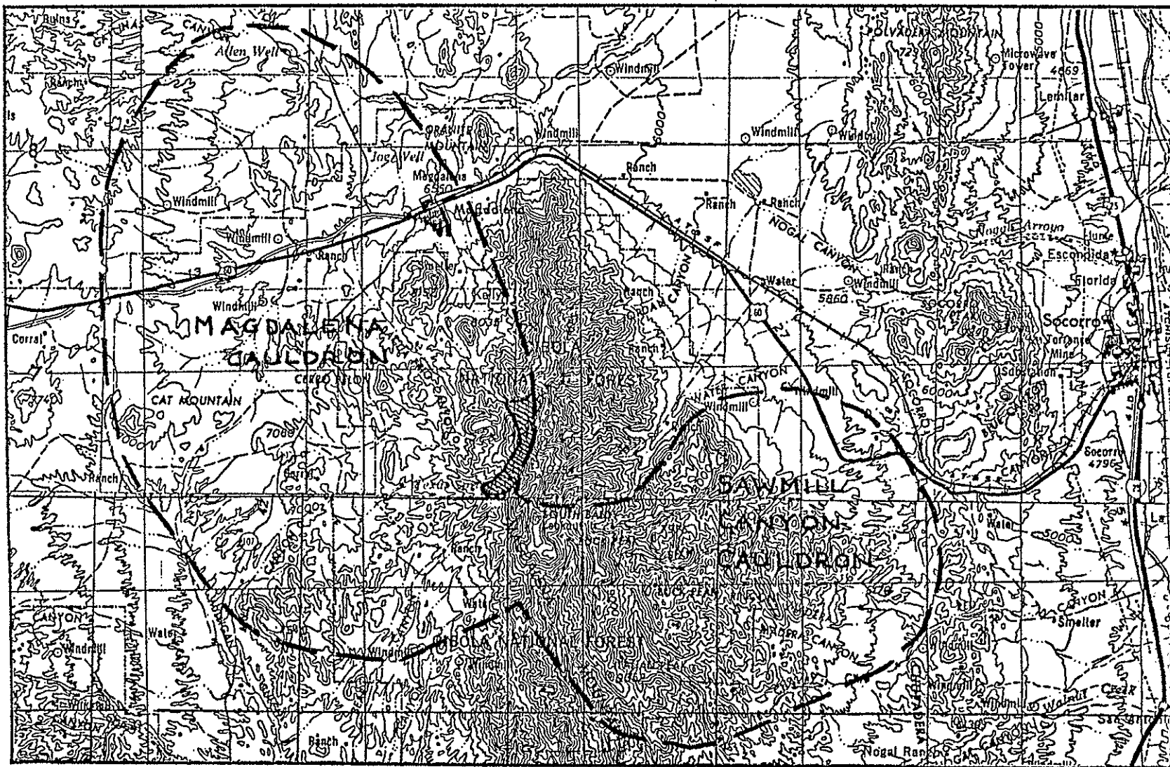
Figure 7. Map showing the relationship between the Magdalena and Sawmill Canyon cauldrons. The area in which Sawmill Canyon cauldron fill crops out in the Magdalena cauldron is shown by hachures.
