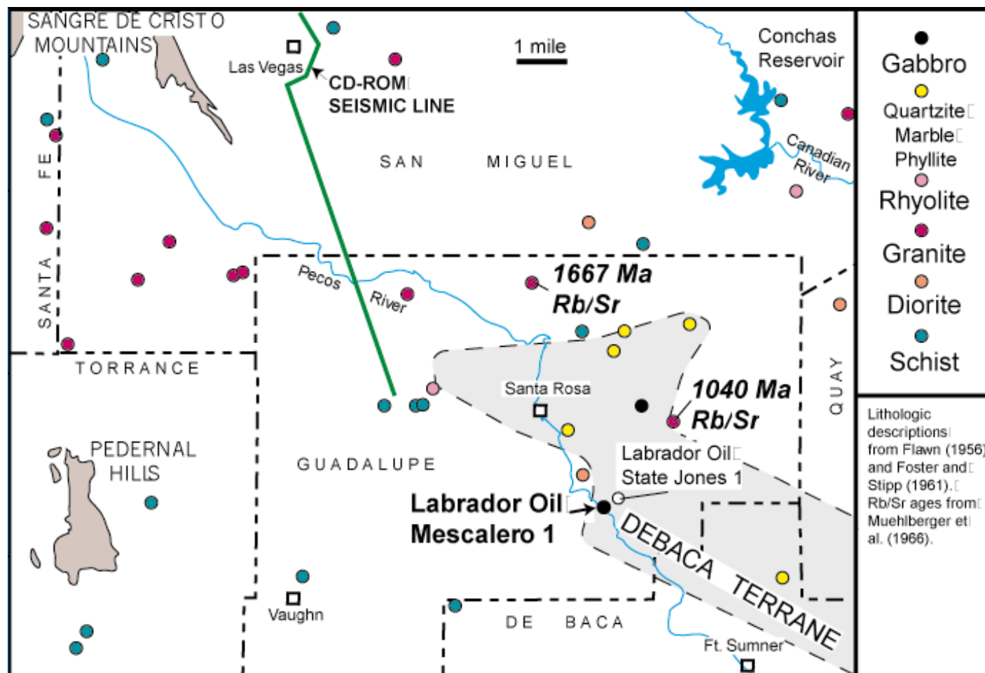
Figure 2. Map showing the location of the Labrador Oil Mescalero No. 1, and other wells drilled in the Tucumcari Basin region. Brown areas are exposed Proterozoic rocks and gray area highlights the Debaca Terrane.
