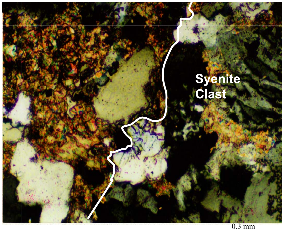
Figure 10. Photomicrograph of meta-arkose showing a clast of quartz syenite (right hand side of the photograph).
