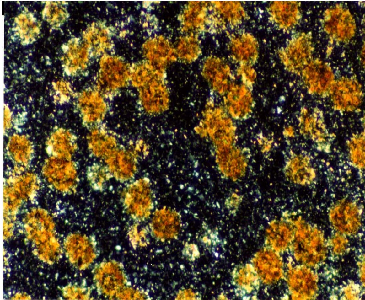
Figure 6- Photomicrograph showing well-developed spotted texture on hornfels suggesting contact metamorphism. Locally, this rock may show relics of plagioclase and re-crystallized quartz crystals. This unit occurs as a thin horizon truncated by two bodies of gabbro at the upper portion of the basement.
