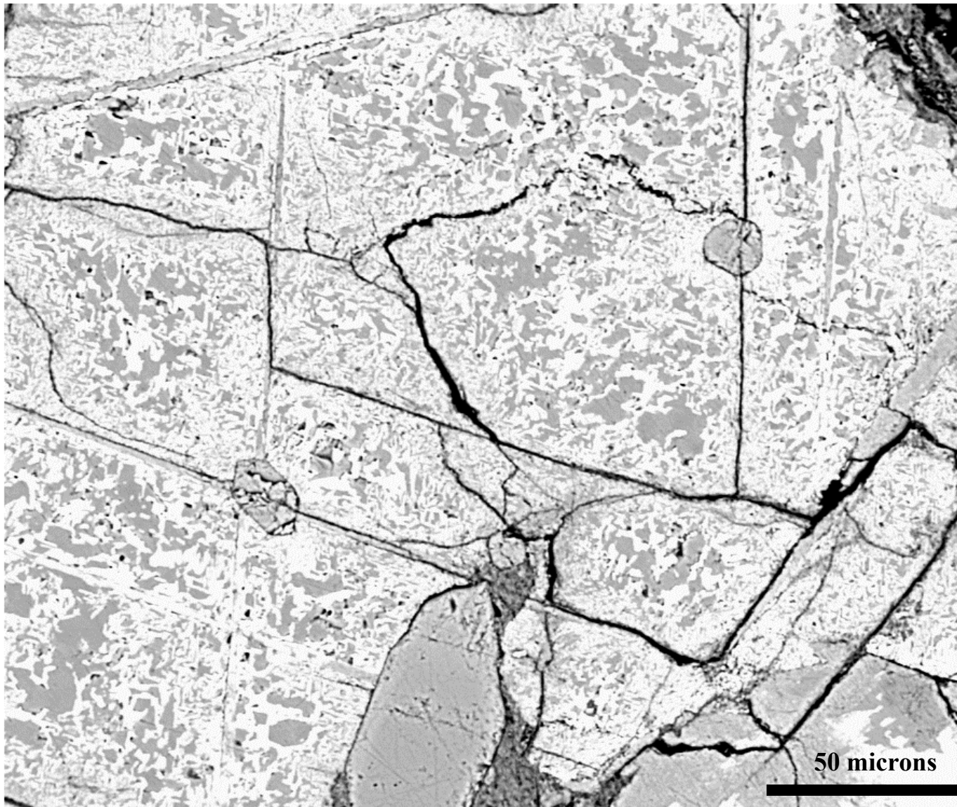
Figure 17. Close up of Figure 16 showing an expanded view of the titanite
