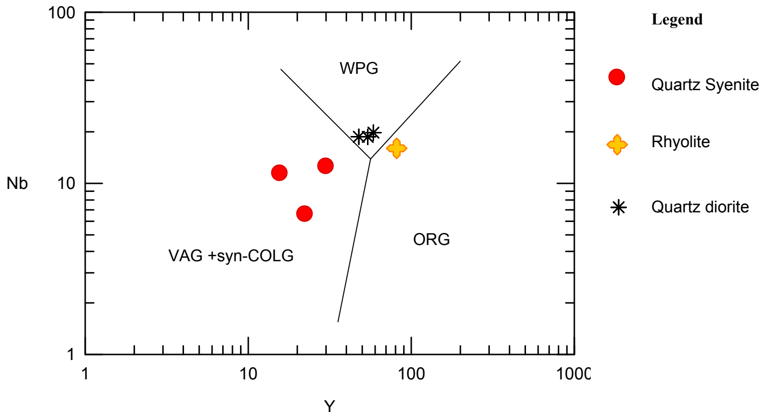
Figure 15A. Nb versus Y discrimination diagram for intermediate and felsic rocks in Mescalero 1. Keys: Syn-COLG is syn-collisional granite; VAG is volcanic-arc granite; WPG represents within plate granite; and, ORG indicates ocean-ridge granite (after Pearce et al., 1984). Values in X and Y axes are expressed in part per million (ppm).
