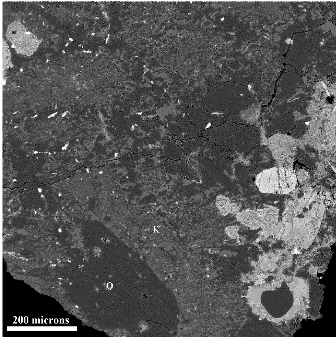
Figure 18. Microprobe Image of quartz syenite showing a graphic texture developed by quartz (Q) and potassium feldspar (K)
