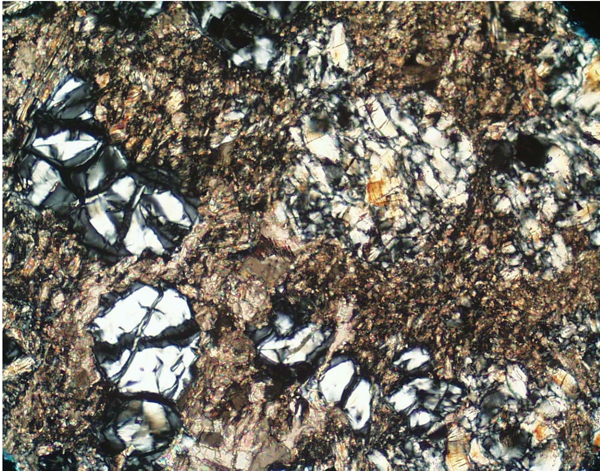
Figure 7- Photomicrograph of tuffaceous metasediment showing zeolitic spherulites (left hand side of the field of view) within a fine-grained groundmass composed mostly by calcite, white phyllosilicate, silica, and clay.
