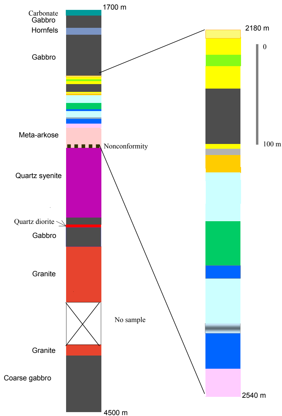
Figure 3. Stratigraphic column of the basement rocks in Mescalero No. 1.
