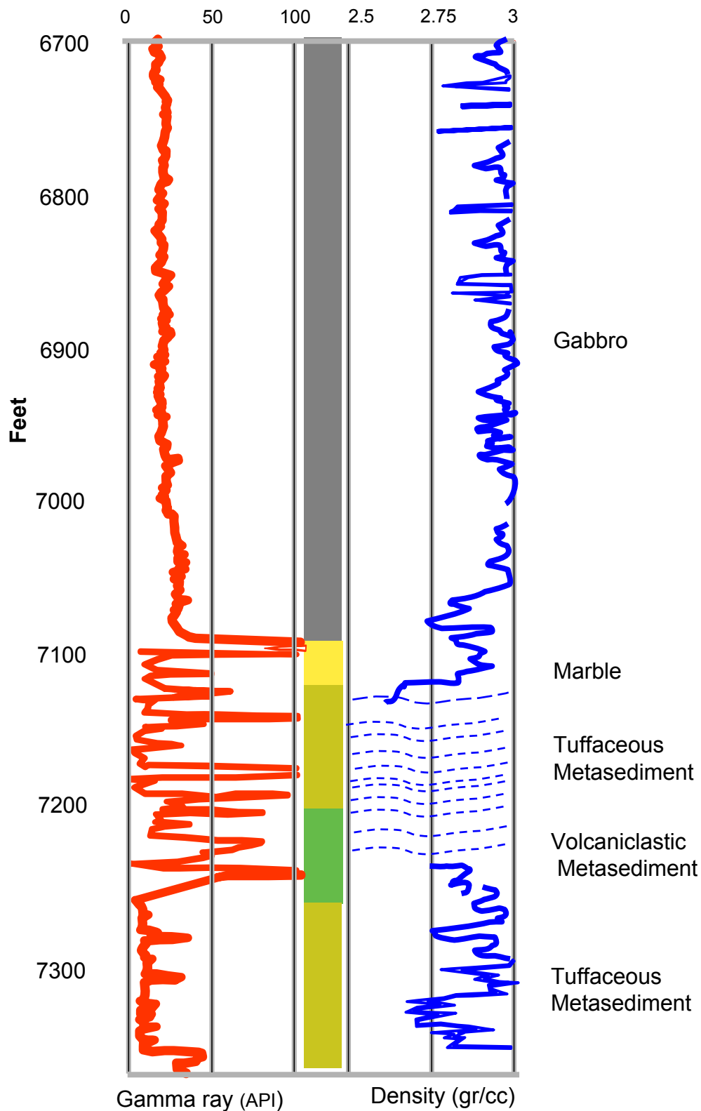
Figure 12. Relationship between lithology, gamma ray activity and density. Keys: The red line represents total gamma ray activity. The blue line on the right side of the diagram represents density. The variability of the density line (wavy shape near the bottom of the diagram) may be an indication of wash out (excessive borehole diameter during drilling) in this interval.
