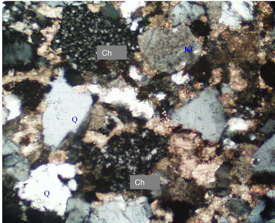
Figure 9. Photomicrograph of meta-arkose. Framework grains consist of quartz (Q), potassium feldspar (Kf) and fragments of chert (Ch). Matrix is composed of mixed carbonate (calcite) and clay. Locally, this unit is rich in fragments of syenite.
