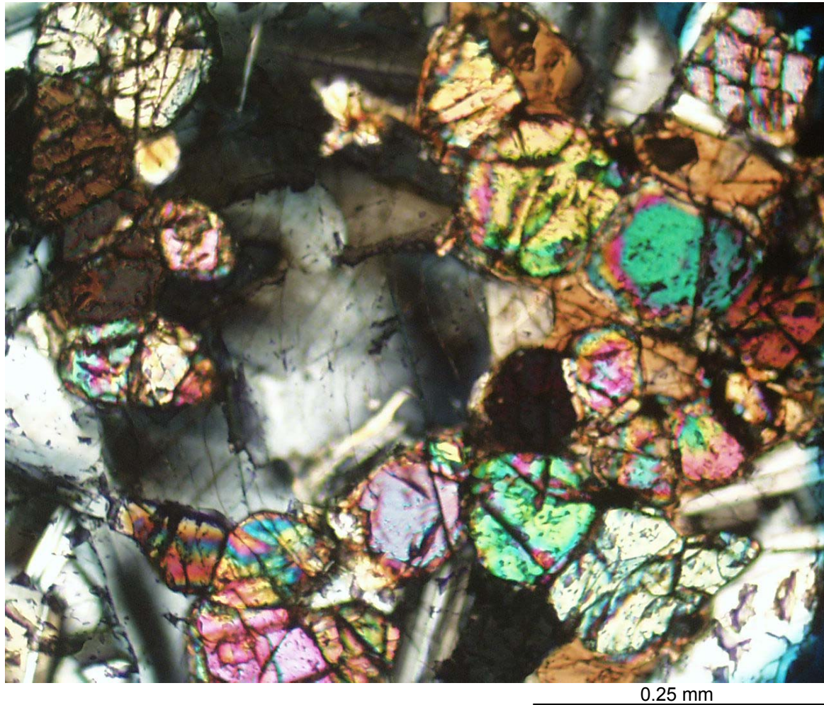
Figure 5. Photomicrograph of gabbro exhibiting a cumulate to subophitic intergrowth texture in which anhedral pyroxene crystals (brown) occupy the spaces between crystals of feldspar, and olivine crystals (greenish, bluish to reddish) of fairly uniform size are developed within the largest crystals of pyroxene.
