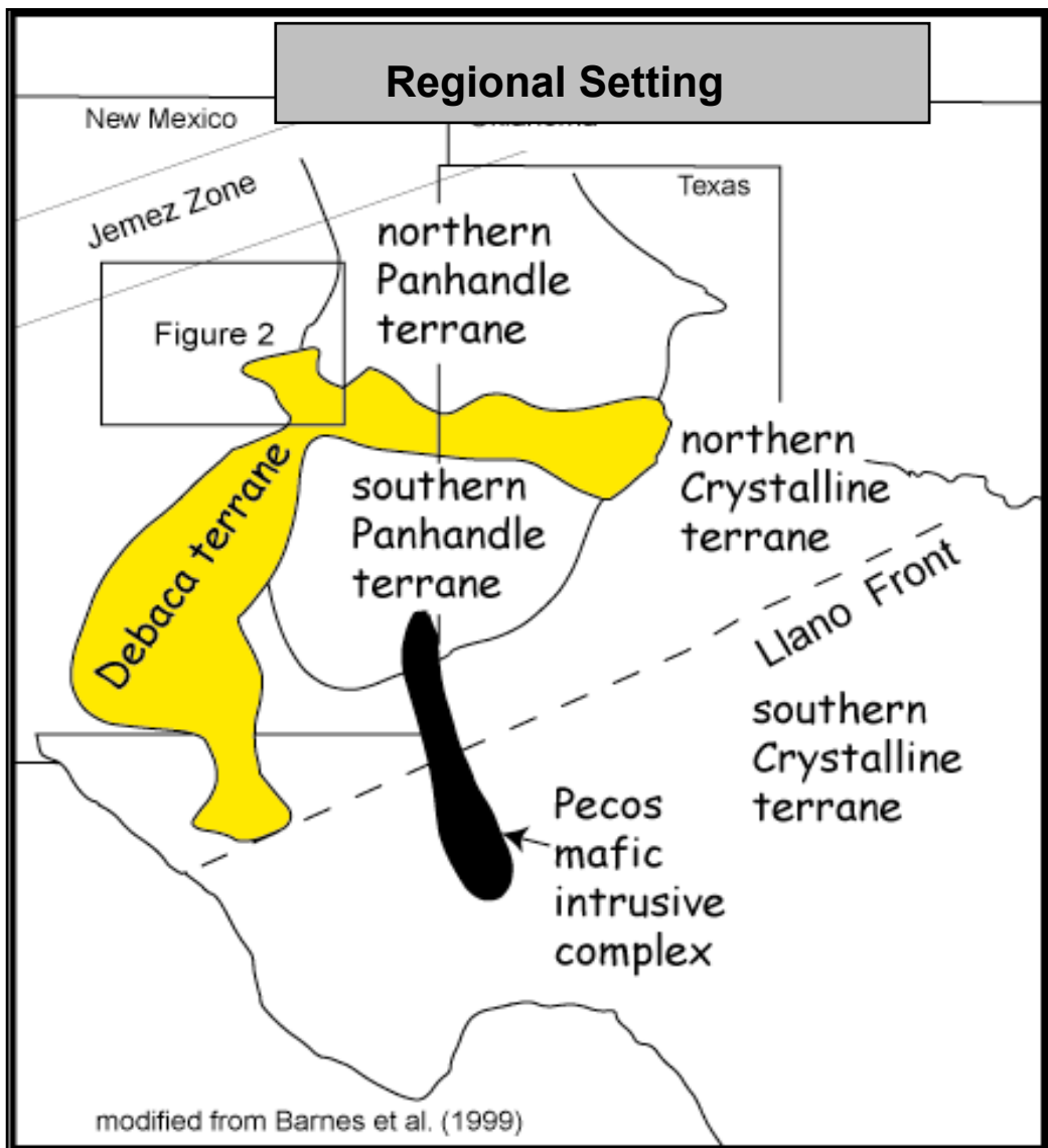
Figure 1. Generalized map showing the location of the Tucumcari Basin with respect to the Proterozoic terranes: the Panhandle Terrane, the Crystalline Terrane, the Pecos Mafic Intrusive Complex, the Llano Front, and the Debaca Terrane.
