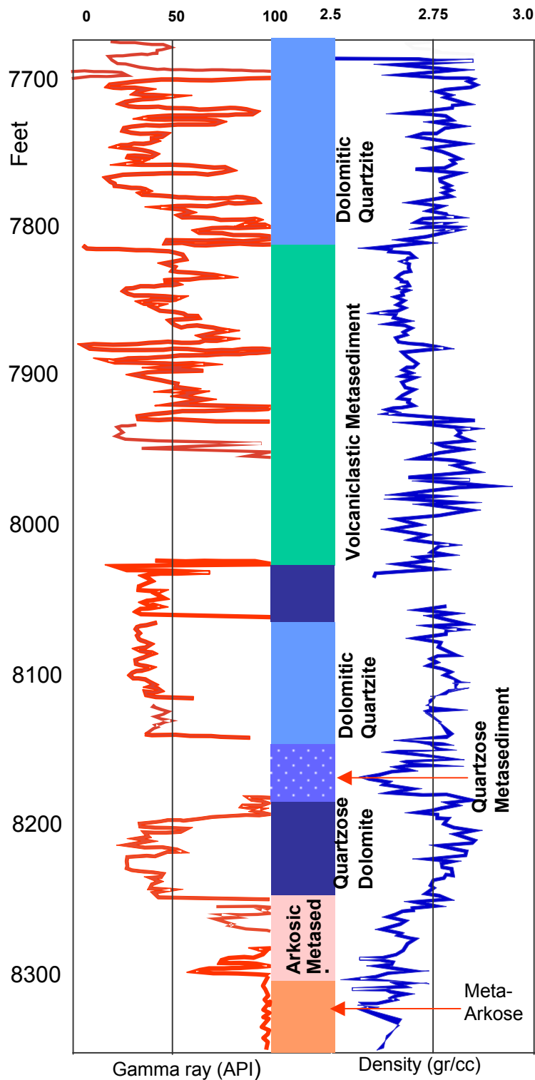
Figure 13. Correlation between lithology, gamma ray activity and density. Keys: The red line represents total gamma ray activity. The blue line on the right side of the diagram represents density. The orange arrows point out two rock types: quartzose metasediment and meta-arkose.
