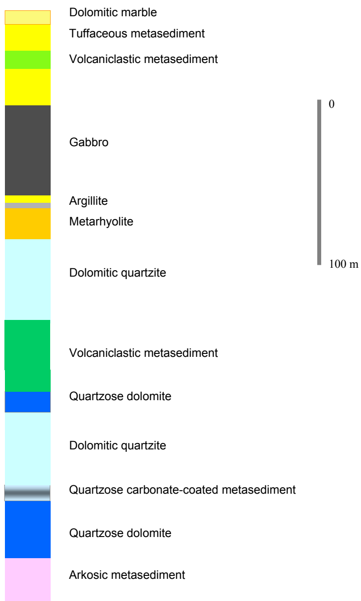
Figure 4. Expansion of the metasedimentary-metavolcanic stratigraphic column.
