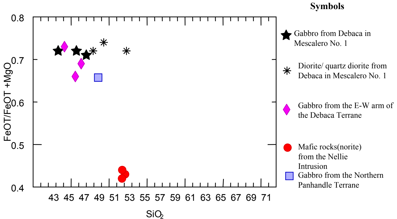
Figure 15. \text{FeO}_T / \text{FeO}_T + \text{MgO} versus \text{SiO}_2 plot for samples of mafic rocks from the E- W arm of the Debaca Terrane in Mescalero 1, Nellie Intrusion, and Northern Panhandle Terrane.
