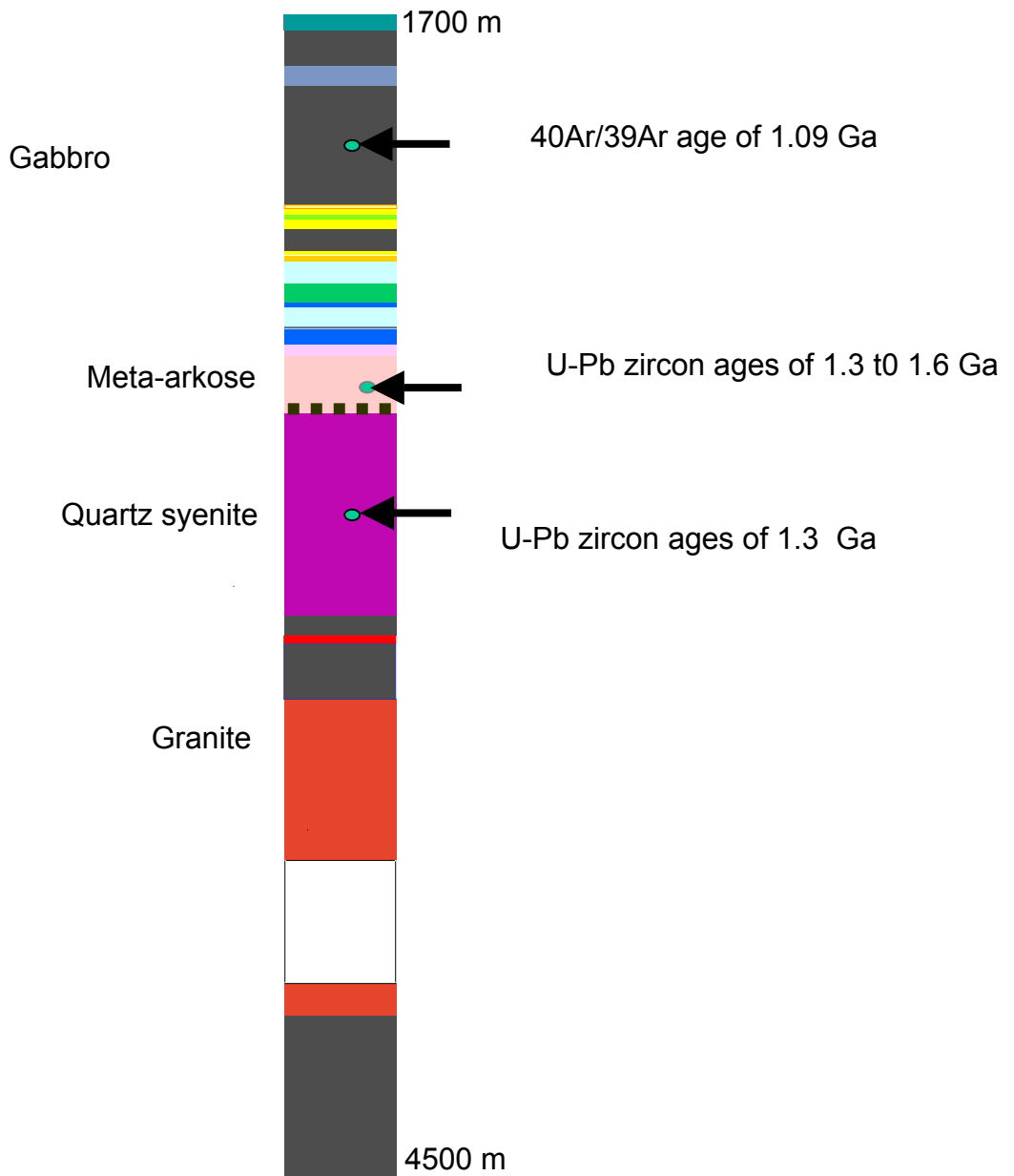
Figure 19. Preliminary results of geochronologic analysis based on ^{40}\text{Ar}/^{39}\text{Ar} and SHRIMP U-Pb zircon methods.
