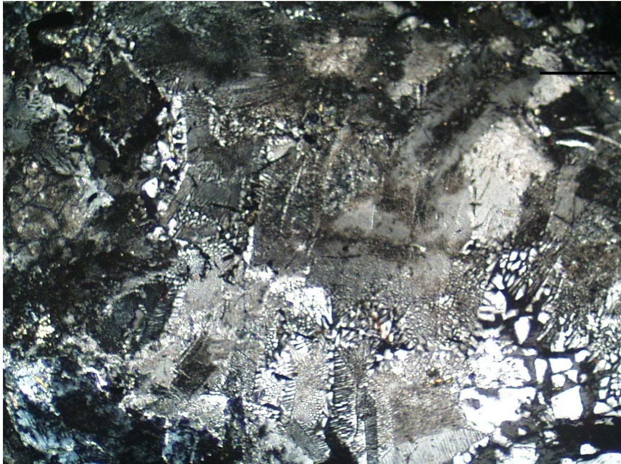
Figure 11. Photomicrograph of quartz syenite showing a granular to granophyric texture with myrmekitic intergrowths of potassium feldspar (gray) and quartz (light-colored) in which quartz forms a wormy texture within the potassium feldspar.
