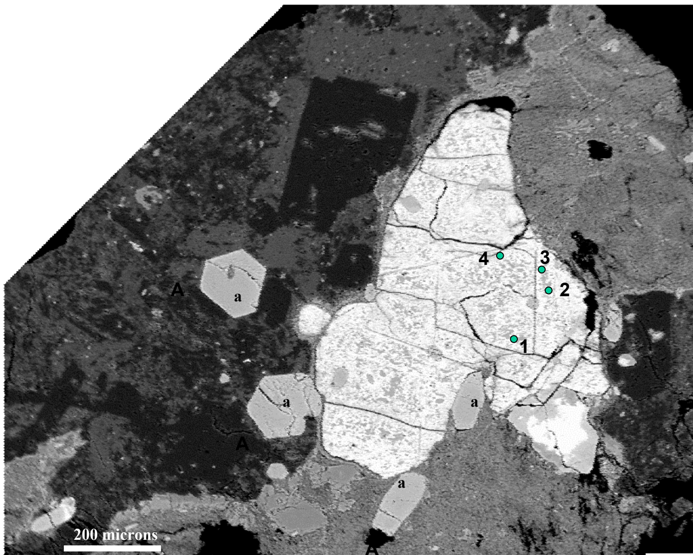
Figure 16. Microprobe image of the quartz zyenite. The grain at center is titanite intergrowths with ilmenite. The euhedral crystals surrounding the titanite are apatite (a).
