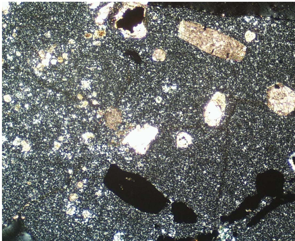
Figure 8- Photomicrograph of meta-rhyolite exhibiting a porphyritic texture in which euhedral hornblende phenocrysts are embedded within a aphanitic groundmass. Note amphibole (upper right) partially replaced by calcite.
