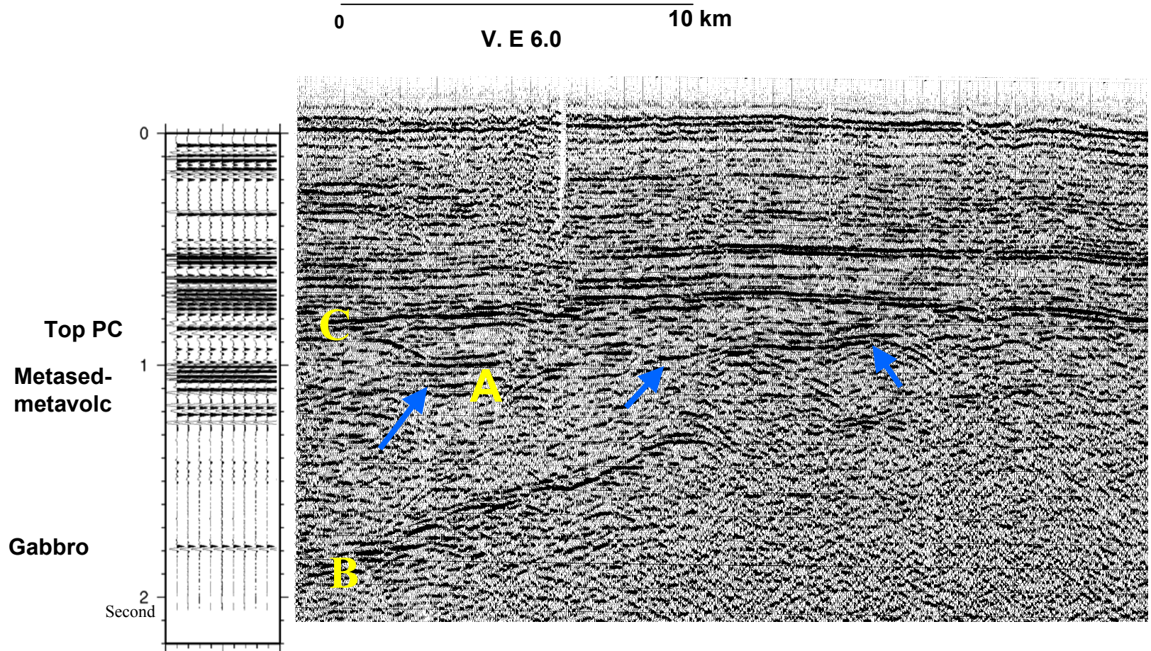
Figure 20. Seismic reflection lines across the Tucumcari Basin, showing strong basement reflectors. The vertical column, on the left of the diagram, is a synthetic derived from the sonic log from a nearby well. Keys: The letter A and highlighted with arrows show base of the Debaca sequence. C represents the top of the Proterozoic basement, and B represents an intrusion of gabbro.
