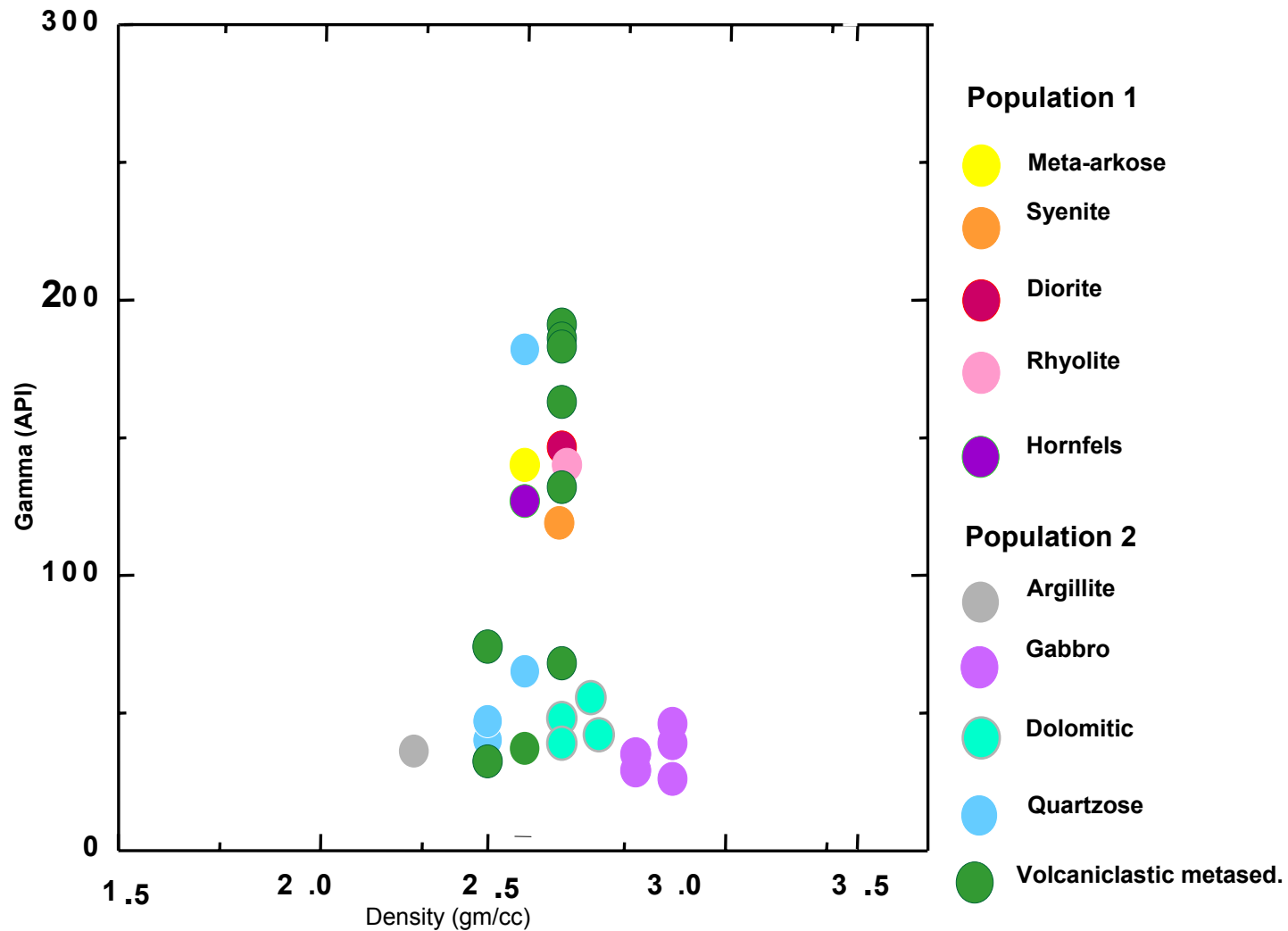
Figure 14. Cross-plot diagram showing the relationship between gamma ray activity and density for different rock types. Values on the Y-axis represent total gamma ray (GAPI) and the values on the X-axis represent density (gm/cc)
