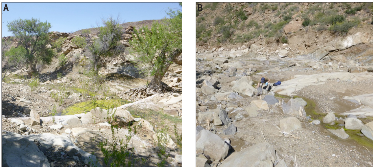
Figure 11. A—Ash Canyon Spring (JM-509) and B—Mescal Spring (JM-500).
