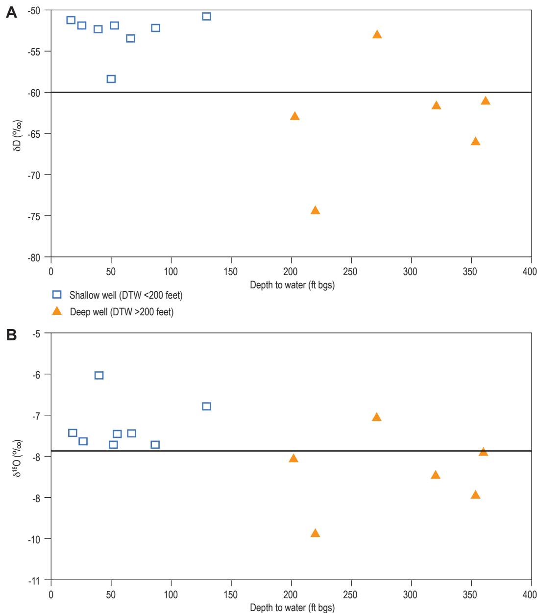
Figure 25. Stable isotopic values (A— \delta D , B— \delta^{18}O ) as a function of depth-to-water. Isotopic compositions of groundwater can be used to differentiate between “deep” and “shallow” waters. Depth to water is in feet below ground surface.
