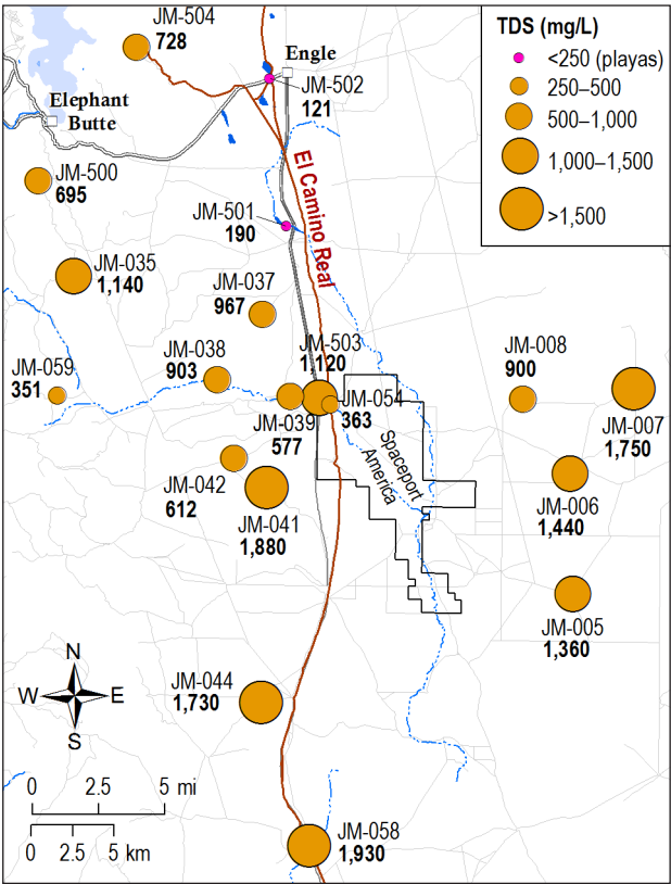
Figure 19. Total dissolved solids in groundwater varies significantly over the study area. In general, the lowest TDS values are found in the center of the study area near the Spaceport America. TDS values increase to the east and south.
