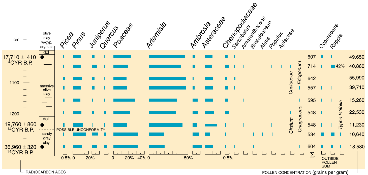
FIGURE 6—Pollen percentage diagram, White Lake, Bailey County, Texas; modified from Hall and Valastro (1995) with new pollen data from late-middle Wisconsinan lacustrine clay.
