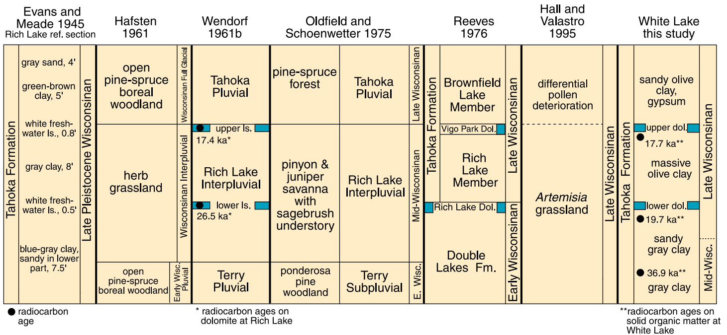
FIGURE 2—Correlation chart of the Tahoka Formation with associated pollen records and selected radiocarbon ages.
