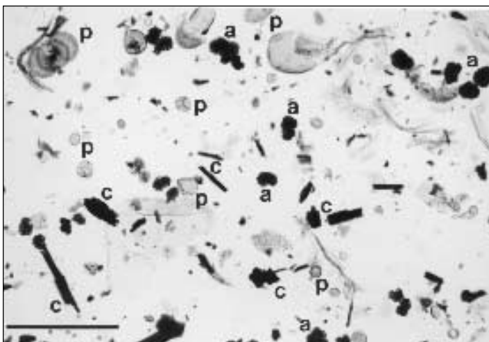
FIGURE 4—Photomicrograph of organic detritus AMS-dated 36,960 ± 320 14 C yrs B.P.; a = algal colony, c = charcoal, p = pollen grain; bar scale = 100 micrometers.
