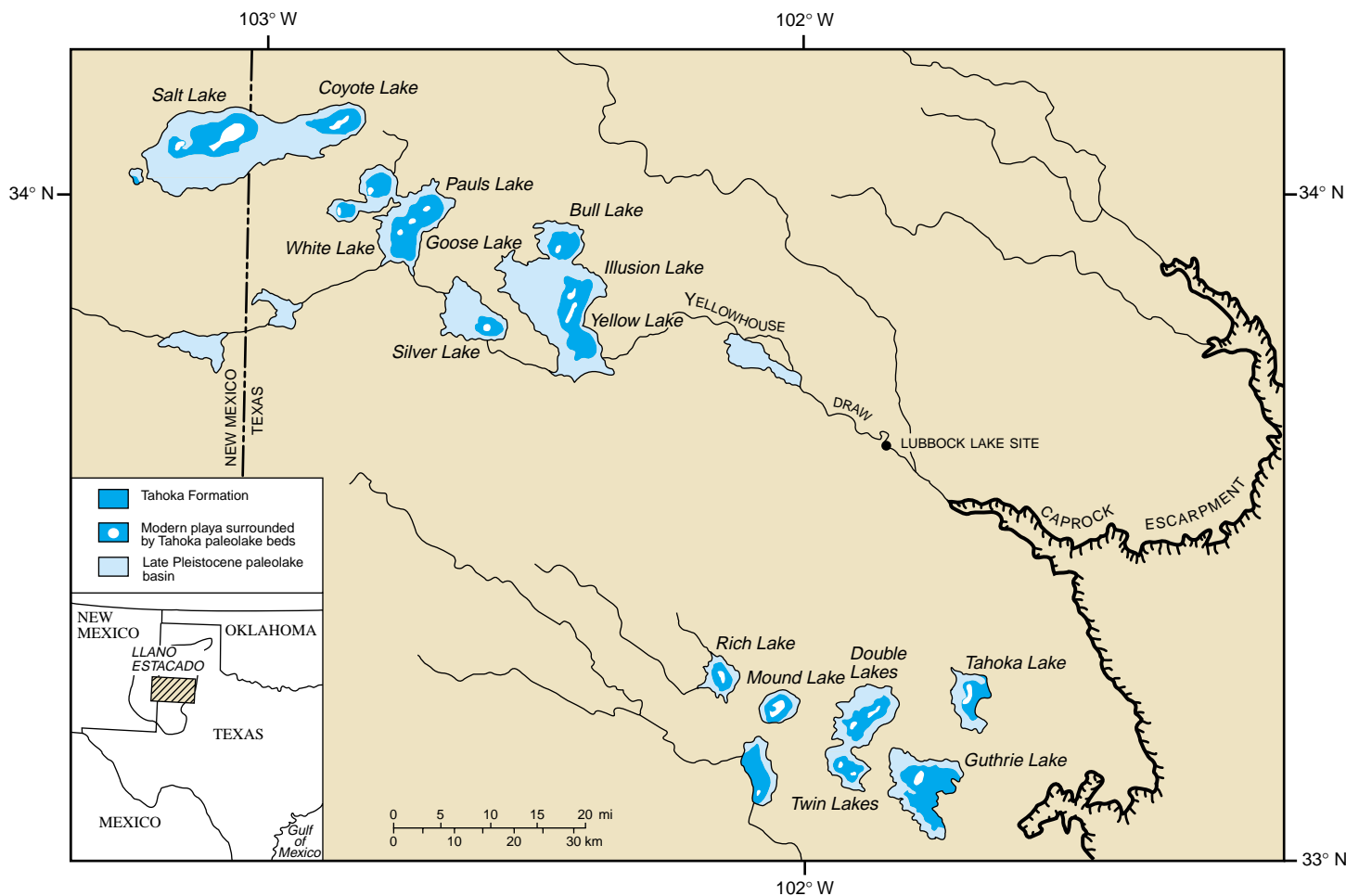
FIGURE 1—Large playa lake basins and the Tahoka Formation on the Llano Estacado, southern High Plains, Texas and eastern New Mexico (modified from Bureau of Economic Geology, 1967, 1968, 1974, 1978).
