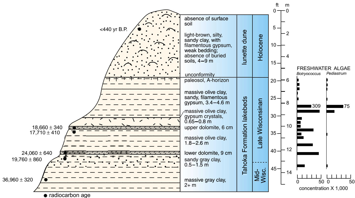
FIGURE 3—Stratigraphy of the Tahoka Formation and overlying lunette dune, measured at the northeast corner of White Lake Basin, Muleshoe National Wildlife Refuge, Bailey County, Texas. Radiocarbon ages are listed
