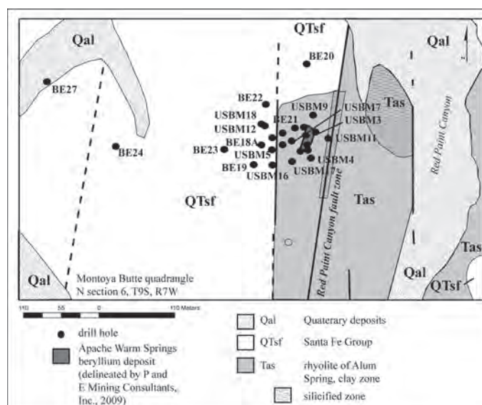
FIGURE 8. Alteration map of the Apache Warm Springs beryllium deposit. The western fault (between BE27 and BE24) is identified from drilling data (McLemore, 2010a).
