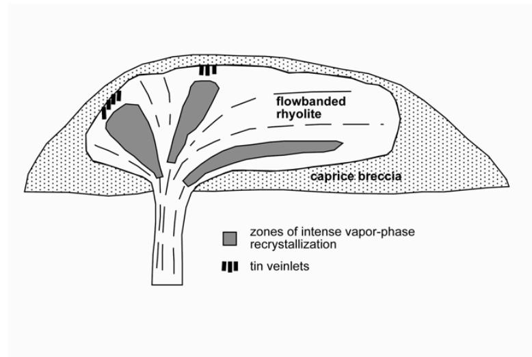
Schematic cross section of flow-banded Taylor Creek dome and associated rhyolite-hosted tin deposits (modified from Eggleston and Norman, 1986).
