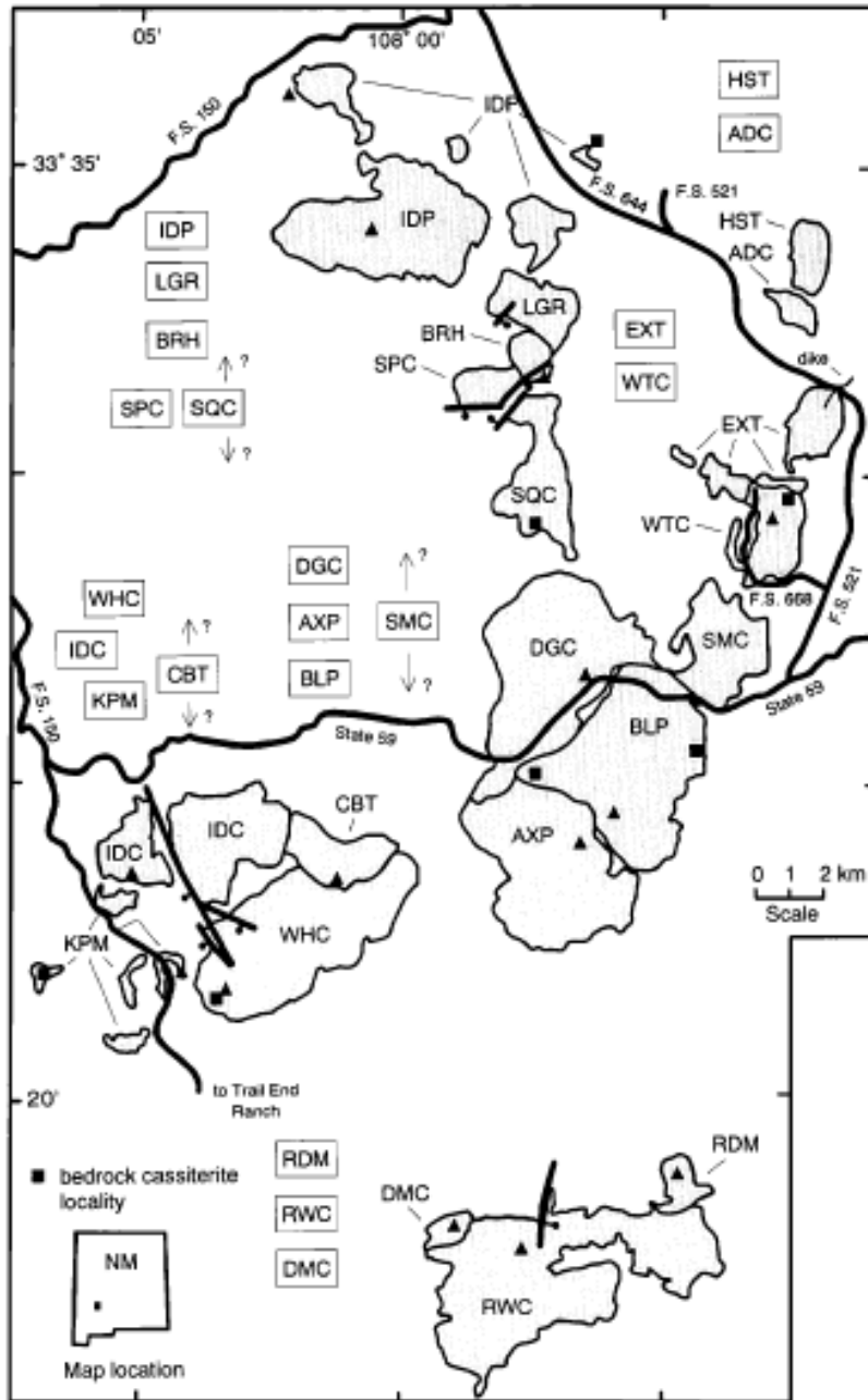
FIG. 1. Geologic map of the Taylor Creek Rhyolite lava domes and flows, after Duffield et al. (1987). Each map unit (e.g., RWC) represents an eruptive unit. Solid triangles indicate sample localities; triangle just outside unit IDP marks sample locality for pumice of initial pyroclastic phase that was followed by emplacement of IDP lava dome. Filled squares represent bedrock cassiterite localities. Bold curves labeled with route numbers are local roads. Relative ages of overlapping units shown by stratigraphic boxes; relative ages of nonoverlapping units unknown. F.S. = unpaved forest service road.
