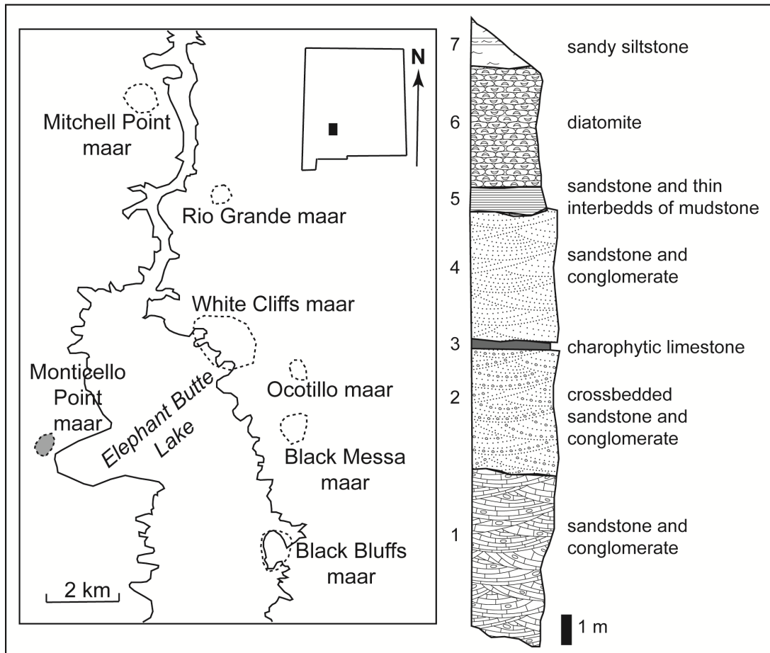
Location and measured stratigraphic column of the Monticello Point diatomite deposit, Sierra County (from Lucas and Kietzke, 1994). Location of maars in the vicinity from Warren (1978).
